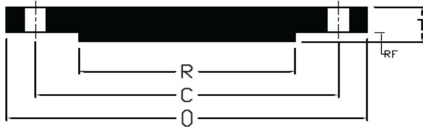
ANSI B16.5 CLASS 1500 BLIND FLANGES
