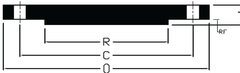
ANSI B16.5 CLASS 150 BLIND FLANGES
