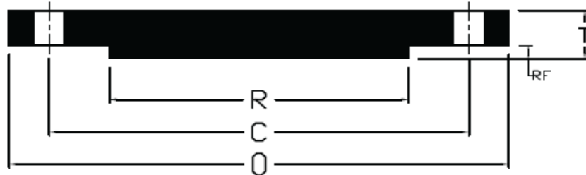
ANSI B16.5 CLASS 300 BLIND FLANGES
