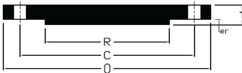
ANSI B16.5 CLASS 900 BLIND FLANGES
