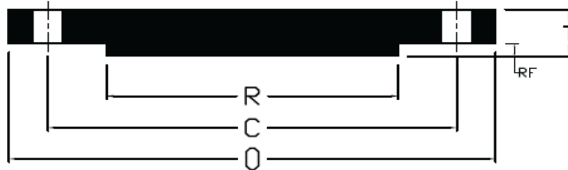
ANSI B16.5 CLASS 600 BLIND FLANGES
