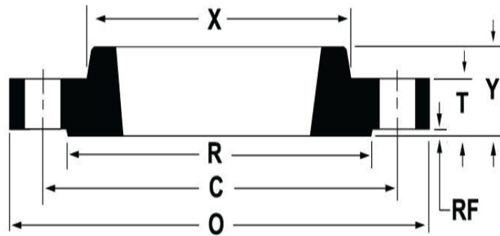
ANSI B16.5 CLASS 900 THREADED FLANGES
