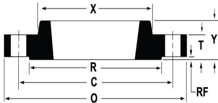
ANSI B16.5 CLASS 600 THREADED FLANGES
