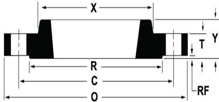
ANSI B16.5 CLASS 150 THREADED FLANGES
