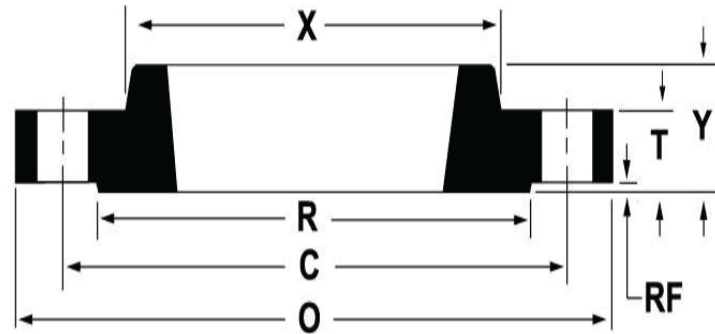
ANSI B16.5 CLASS 300 THREADED FLANGES
