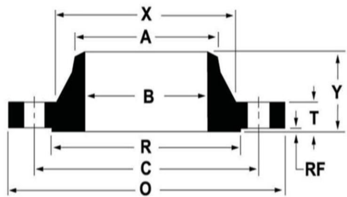
ANSI B16.5 CLASS 150 WELDING NECK FLANGES
