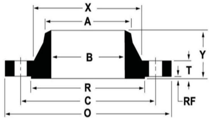
ANSI B16.5 CLASS 900 WELDING NECK FLANGES
