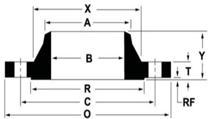
ANSI B16.5 CLASS 300 WELDING NECK FLANGES
