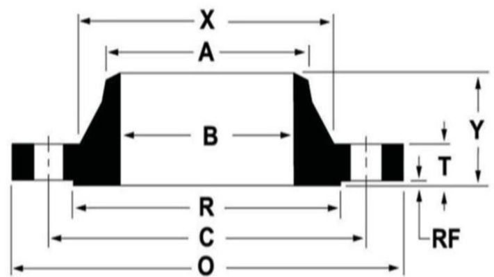
ANSI B16.5 CLASS 1500 WELDING NECK FLANGES
