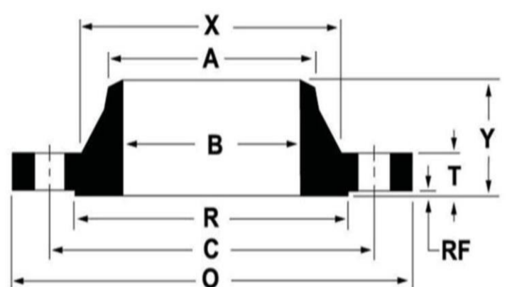
ANSI B16.5 CLASS 600 WELDING NECK FLANGES
